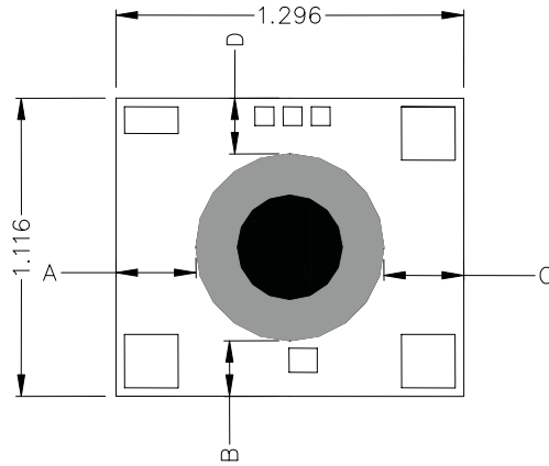
Figure 3-4. Ink Dot Drawing
